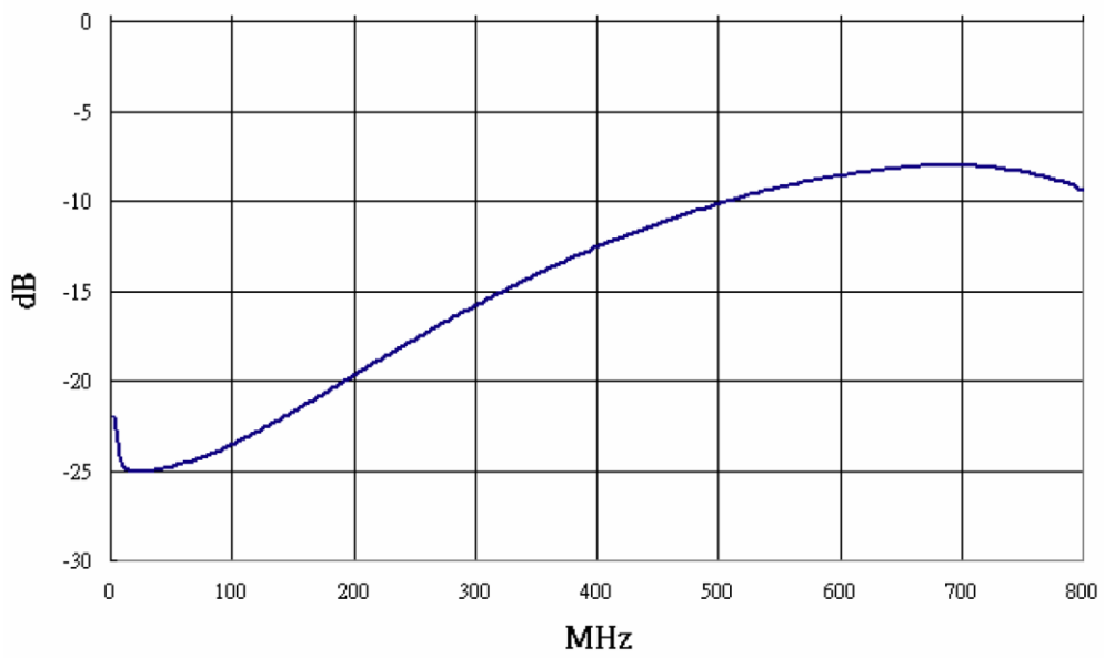
Input Return Loss
